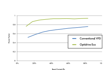
Power factor comparison
