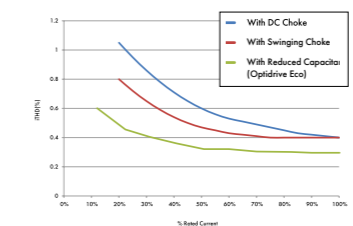
Typical iTHD values at full and part load
